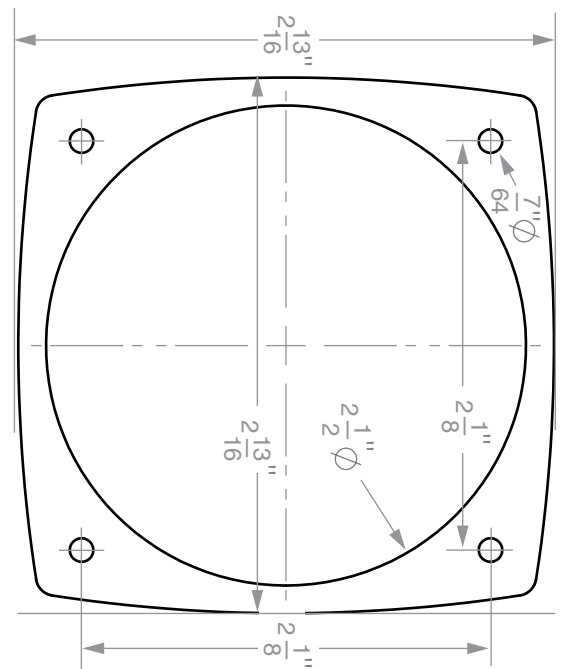
BCI or AutoTrim Pro Control Templates
