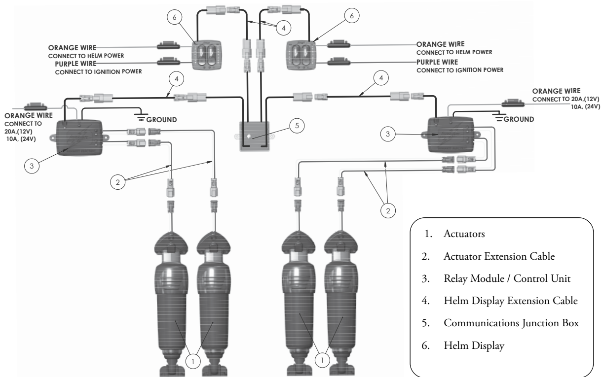
Dual BCI/ATP Display & Dual Actuators
