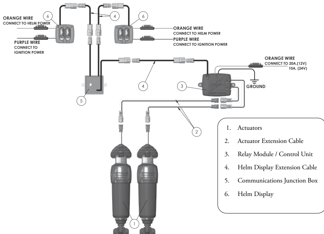
Dual BCI/ATP Display & Single Actuators
