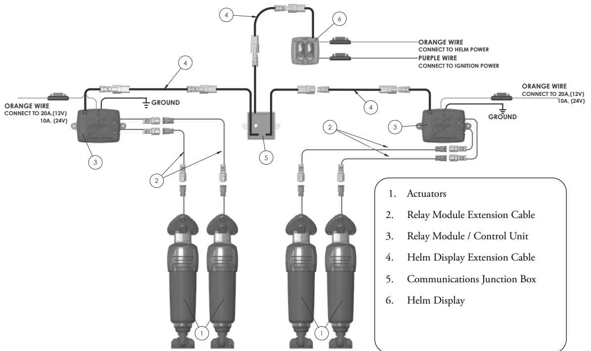
Single BCI/ATP Display & Dual Actuators
