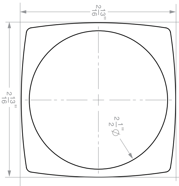
OBI Control Templates
