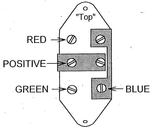
Hatch Lifter Control Wiring Diagram Yellow Wire Is Not Used
